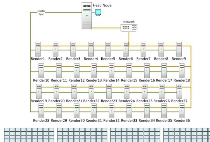
Figure 3: CAVE2 visualization system with 36 computers, 1 head node and 72 displays, networked together.
